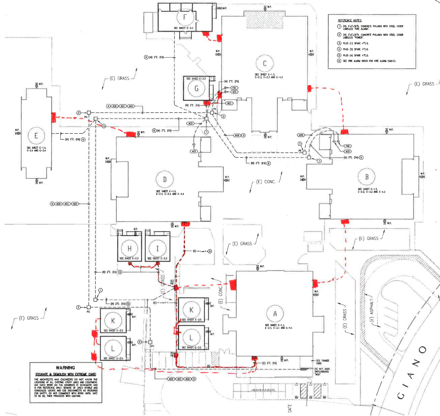
ELECTRICAL SITE PLAN SCALE: 1" = 30'-0"
